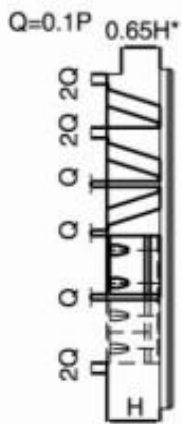
Unit Element Fender Clearance
